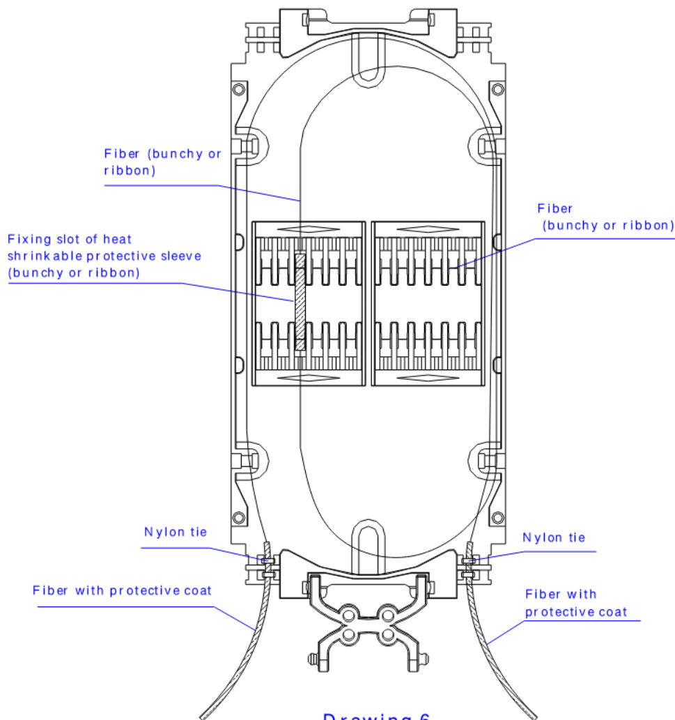
Drawing 6
